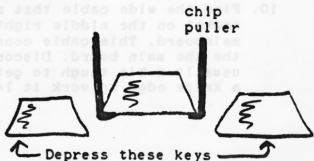
Removing Keycaps
